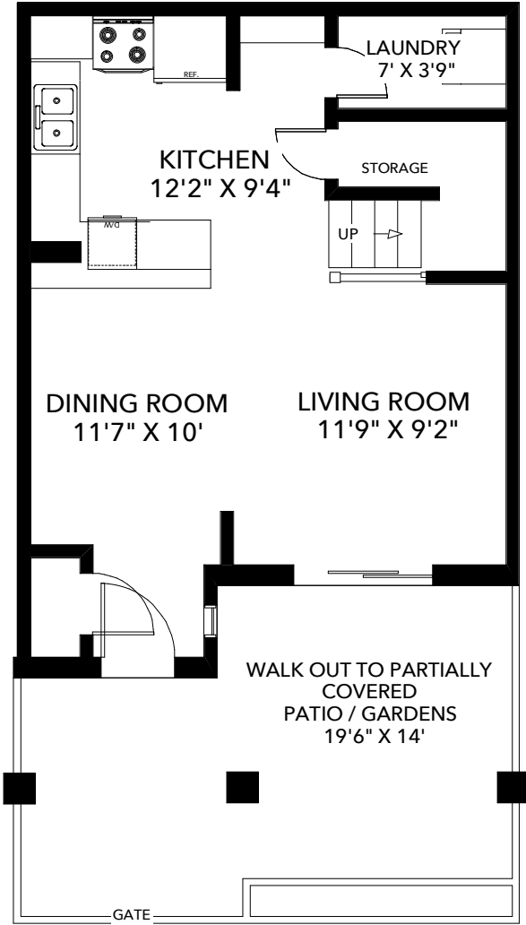
MAIN FLOOR CEILING HT 8'
